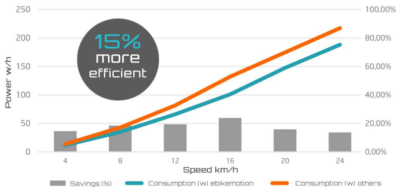
Ebikemotion Smart Controller Consumption
